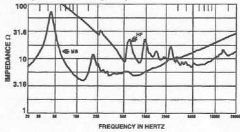
FIGURE 2 — Impedance vs. Frequency
